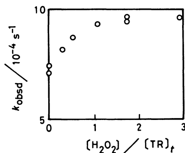
Fig. 6. Relation between k_{\text{obsd}} and ratio of hydrogen peroxide to triose reductone in the presence of oxygen at \text{pH } 6.6 \pm 0.2 and 30^\circ\text{C} .
