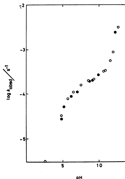
Fig. 5. Relation between \log k and pH for the oxidation of triose reductone with hydrogen peroxide in the presence of oxygen at 30 °C.
