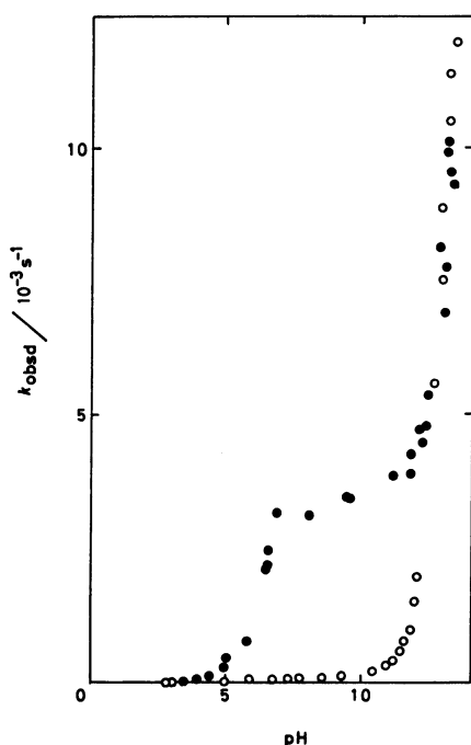
Fig. 3. Relation between k_{\text{obsd}} and pH for the autoxidation of triose reductone in the presence and absence of EDTA at 30 °C.
