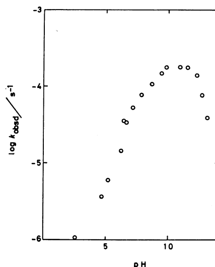
Fig. 4. Relation between \log k_{\text{obsd}} and pH for the oxidation of triose reductone with hydrogen peroxide in the absence of oxygen at 30 °C.
