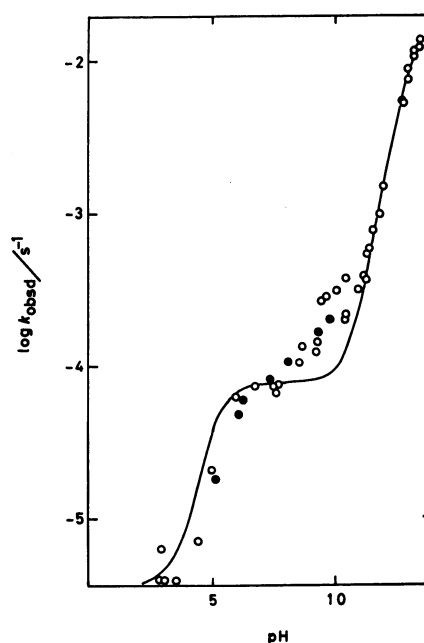
Fig. 2. Relation between \log k_{\text{obsd}} and pH for the autoxidation of triose reductone at 30 °C.
